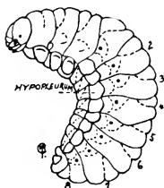
Fig. 351. Pine gall weevil, Podapion gallicola Riley.
